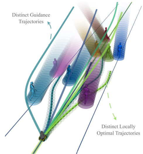
Fig. 1. T-MPC first computes distinct guidance trajectories in the state space (time is visualized in the upwards direction). Each guidance trajectory initializes a local planner, resulting in several distinct locally optimized trajectories. The locally optimized trajectories each pass the obstacles (predicted future motion visualized as cylinders) in a distinct way.
