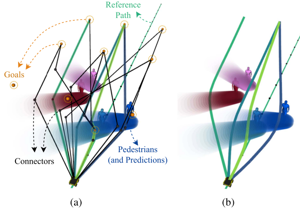
Fig. 4. Illustration of the guidance planner in the state space (time in the upwards axis). Visualization follows Fig. 3. (a) Visibility-PRM graph (black lines and dots) explores the free space toward the goals placed at t = T around the reference path (orange dots). The homotopy distinct guidance paths (colored lines) are obtained by searching the graph. (b) Final trajectories are smoothed.
