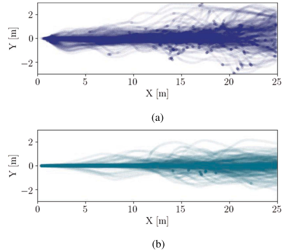
Fig. 8. Trajectories of 200 experiments with 12 pedestrians for the TEB-Planner and T-MPC++. Our method results in smoother and more consistent robot navigation. (a) TEB-Planner [8]. (b) T-MPC++ (ours).
