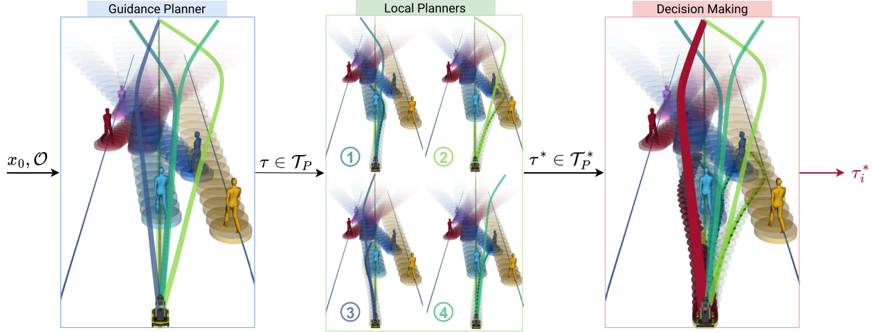
Fig. 3. Schematic of T-MPC. An environment with several obstacles and a robot is visualized in x, y, t (time in the upwards axis). Obstacle motion predictions are denoted with cylinders. 1) A guidance planner (see Section IV-A) finds P = 4 trajectories (visualized with colored lines) from the robot initial position to one of the goals. Each of these trajectories is in a distinct homotopy class in the state space. 2) Each trajectory guides a local planner (see Section IV-C) as initial guess and through a set of homotopy constraints. Four guidance trajectories and optimized trajectories (as occupied regions for each step) are visualized. 3) The optimized trajectories are compared through their objective value (see Section IV-E) and a single trajectory (in red) is executed by the robot.
