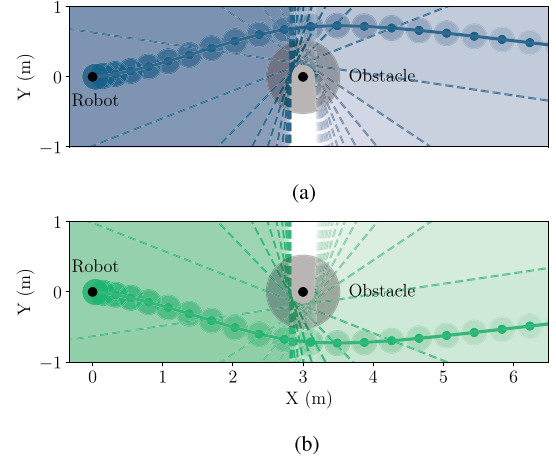
Fig. 5. Two distinct locally planned trajectories for a robot (black dot) evading an obstacle (black region and dot) that is static ( \mathbf{o}_k = \mathbf{o}_0, k = 1, \dots, N ). For both planners, we depict the topology constraints for each time step in their respective colors showing the constraint boundaries (broken lines) and their feasible region (colored regions with increasing transparency over time). (a) Local planner 1 plans to evade the obstacle left. (b) Local planner 2 plans to evade the obstacle right.
