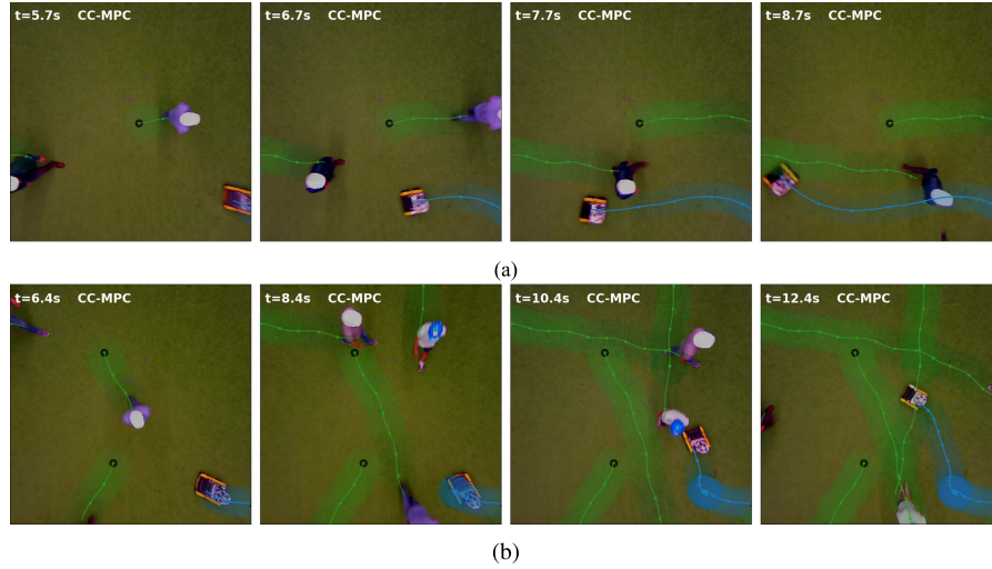
Fig. 13. Trajectories of baseline CC-MPC [4] overlaid on camera images. Black dots denote pedestrian start positions. (a) Baseline fails to find the more efficient trajectory passing between two incoming pedestrians. (b) Baseline becomes infeasible and does not recover quickly (note the time scale).
