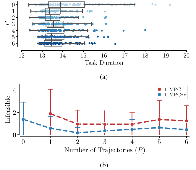
Fig. 9. Sensitivity study of the number of guidance trajectories P . (a) Task duration of T-MPC++, individual experiments denoted by dots. (b) Mean and standard deviation of the number of control iterations in which the optimization is infeasible per experiment (out of approximately 280 iterations each) for the same simulations. (a) Task duration of T-MPC++. (b) Infeasible iterations (mean and std) per experiment.
