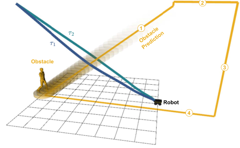
Fig. 15. Illustrating example for the H-signature [30]. The two trajectories \tau_1 (blue) and \tau_2 (green) are in distinct homology classes as the loop that they form contains obstacle skeleton (orange). In practice, link (3) is placed far away.
