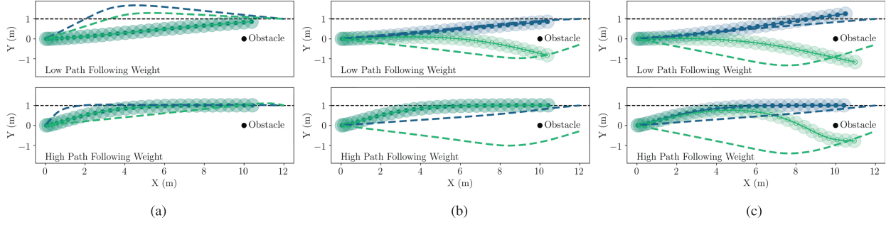
Fig. 6. Planned trajectories (lines with shaded discs) tracking a reference path (dashed black line) while avoiding a static obstacle with two guidance trajectories (dashed lines) for a low (0.01) and high (0.3) path following weight. (a) Without homotopy comparison (3), guidance trajectories are not distinct and optimized trajectories are identical. (b) Without homotopy constraints, increasing the path following weight results in identical trajectories. (c) With homotopy comparison (3) and homotopy constraints (9e), optimized trajectories are distinct. (a) Without homotopy comparison (3). (b) Without constraints (9e). (c) Our proposed method.
